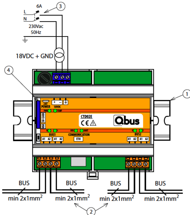
Figure 2 : Connection controller CTD02E
