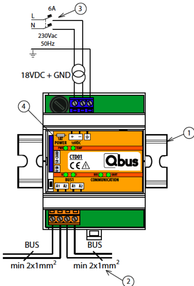
Figure 2 : Connection controller CTD01
