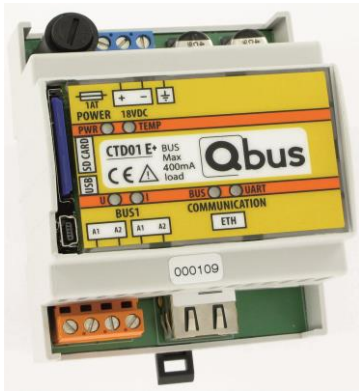
Figure 1 : Controller CTD01E+
