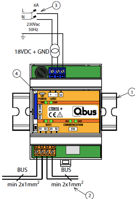
Figure 2 : Connection controller CTD01E+
